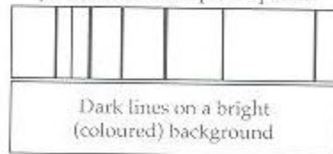
▲ Fig 18.14 Electron transitions from a lower to a higher energy state in a hydrogen atom
